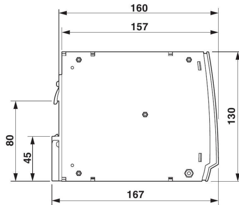
Figure 3 Device dimensions
