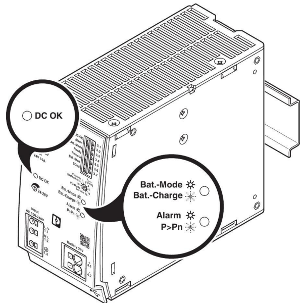
Figure 37 LED indicators
