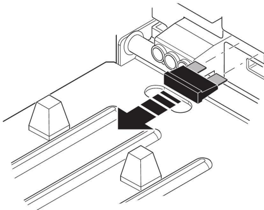
Figure 28 Remove fuse
